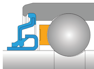
TRIPLE LIP SEAL
