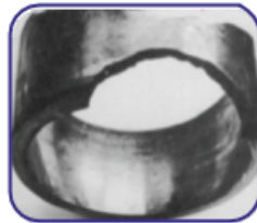
Fatigue fracture of an outer ring from snap ring groove in Double Row Angular Contact Ball Bearing caused by axial loading
