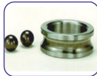
Fluting on inner ring raceway with dark colored balls
