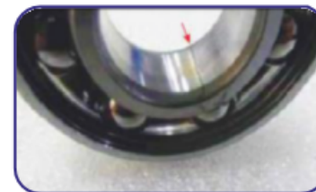
Forced fracture due to excessive interference fit
