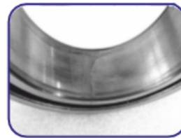
Thermal cracking on cone bore of taper roller bearing
